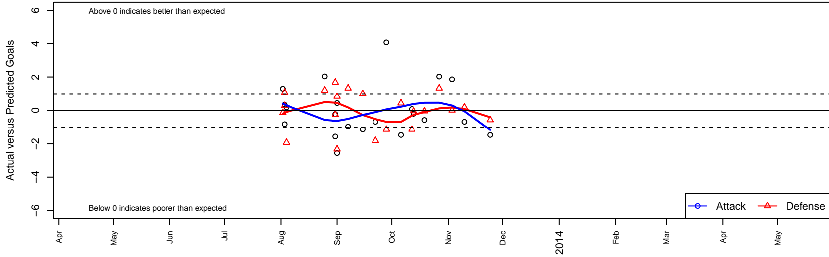
Whatcom Select B95 Dots are actual minus expected GF (blue circles) and GA (red triangles). Blue line is smoothed change in attack strength. Red is smoothed change in defense strength.
